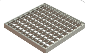
Gratar OZ BASIC grila pt camin patrat A15 300x300 (3320)
